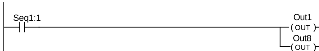
Figure 3.10 - Circuit #3
